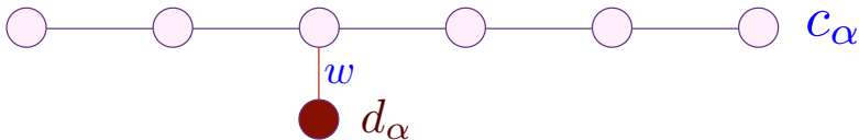
FIG. 1. Resonant level model of free electrons: conduction electrons c_\alpha hybridize with a localized d_\alpha state with amplitude w . The c_\alpha move on a d > 1 dimensional lattice, although only one dimension is shown.
