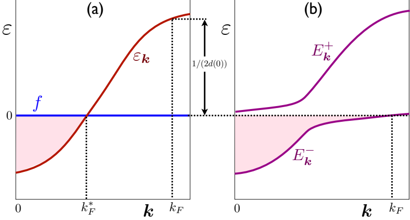
FIG. 9. Schematic band structures in the FL and FL* phases. In (a), we show the conduction electron band \varepsilon_{\mathbf{k}} , and the decoupled f band at zero energy; the conduction electron states with energy \varepsilon_{\mathbf{k}} < 0 are occupied and have density \rho_c , while the f band is half-filled. The HFL state is obtained when the mixing between the bands is non-zero (given by \bar{P} in (69)), and the f band is shifted by \bar{\lambda} in (67). This results in the bands shown in (b). Only the lower band in (b) is occupied, up to the wavevector k_F , for a total density of 1 + \rho_c . The values of k_F in (a) and (b) are the same, with the value of \varepsilon_{k_F} specified by (70).
