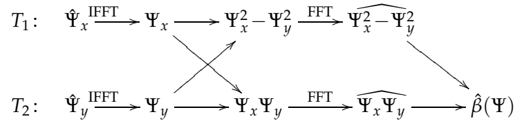
Figure 6: Data flow for computing the non-linear term.
