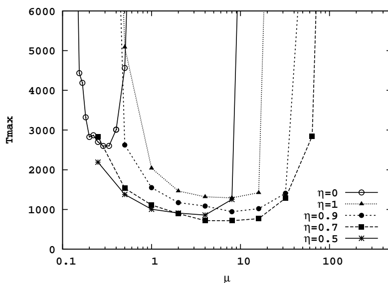
Figure 4: T_{\max} versus \mu where \epsilon = 10^{-10} , T = 25000 and K = 10 . Note that T_{\max} is the time after which the approximate solution remains within \epsilon of the reference solution, K^2 is the resolution of the observations and \eta is the smoothing parameter in the interpolant.
