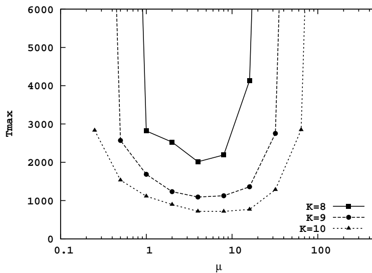
Figure 5: T_{\max} versus \mu for \epsilon=10^{-10} , T=25000 and \eta=0.7 . Note that T_{\max} is the time after which the approximating solution remains within \epsilon of the reference solution, K^2 is the resolution of the observations and \eta is the smoothing parameter in the interpolant.
