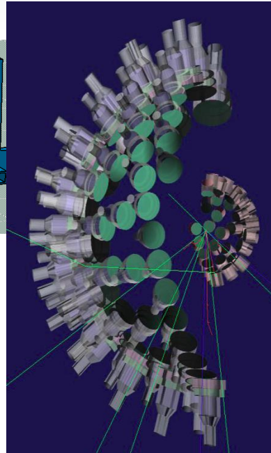
Gamma above neutron threshold
