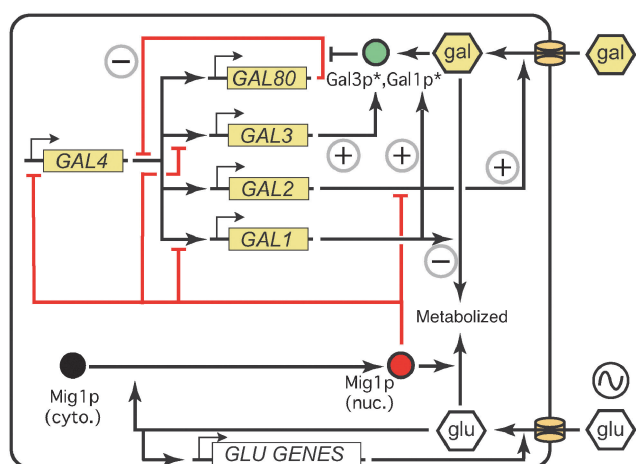
Fig. 1 The GAL network is controlled by interlocking positive and negative feedback loops. Asterisks indicate activation by intracellular galactose. Red indicates repressive effects; green represents inducers. Positive and negative feedback loops are marked with circled + and – signs, respectively. See text for details. Adapted with permission from ref. 29.
