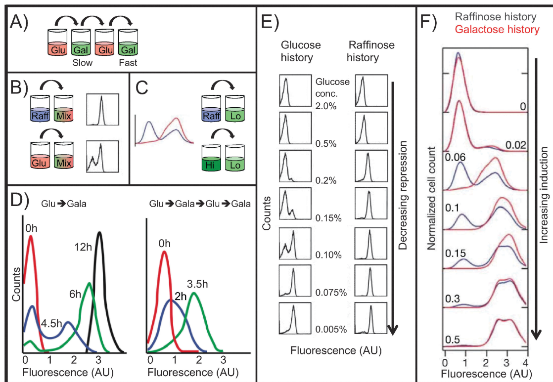
Fig. 3 Reinduction and persistent memory. All histograms are flow cytometry measurements of single-cell fluorescence intensity of GAL gene reporters. Fluorescence intensity is on a \log_{10} scale. All strains are wild-type except for GAL reporters. (A) Reinduction memory experiment (12-hour): 4 glucose, galactose (slow GAL induction), glucose, galactose (fast GAL induction). (B) Persistent memory experiment: 5 raffinose or glucose, then a mix of galactose and glucose (14 h). (C) Persistent memory experiment: 6 raffinose or high galactose, then low galactose (27 h). (D) Reinduction memory data. Timecourses of Gal1p-GFP fusion protein expression in cells growing in 2% galactose media. Left: initial galactose induction after pre-growth in glucose (> 24 h). Right: reinduction in galactose after pre-growth in glucose (> 24 h), galactose (24 h), and glucose again (12 h). The second induction is faster and unimodal, demonstrating reinduction memory. Adapted with permission from ref. 4. (E) Persistent memory under weak repression, showing the effects of pre-growth history in glucose vs. raffinose. Following the pre-growth phase, cells were grown for 14 h in 2% galactose plus the indicated concentration of glucose. Flow cytometry measurements show the fluorescence intensity of a GFP reporter of GAL1 promoter activity. In moderately repressing medium (center images), glucose-history cells are bimodally distributed; raffinose-history cells are unimodal and the ON peak displays a graded response to glucose repression. Adapted with permission from ref. 5. (F) Persistent memory under weak induction, showing the effects of pre-growth for 12 h in raffinose (blue) vs. 2% galactose (red). After pre-growth, cells were grown for 27 h in the indicated concentration of galactose. Flow cytometry measurements show the fluorescence intensity of a YFP reporter of GAL1 promoter activity. Raffinose-history cells are bimodally distributed; galactose-history cells are unimodal and display a graded response to galactose concentration. Adapted with permission from ref. 6.
