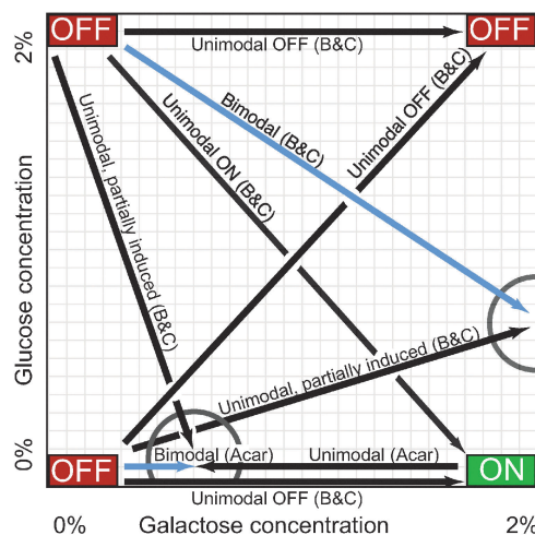
Fig. 4 The carbon landscape. The arrows summarize persistent memory experiments described in the text, which measured GAL1 reporter expression at various concentrations of galactose ( GAL inducer) and glucose ( GAL repressor) in wild-type yeast. Drawing is not to scale. "OFF" and "ON" refer to the expression level of GAL1 at the extremes of glucose and galactose concentration. Cells were incubated in one carbon source (arrow bases) and then transferred to a new medium (arrowheads) for 14–27 h. Blue arrows indicate bimodal expression in the new medium, i.e., some cells are induced and others are not. Black arrows indicate a homogeneous (unimodal) cell population in the new medium. Partial circles highlight points on the carbon landscape where cellular memory of the sugar (carbon source) history affects steady-state GAL expression in the new medium (i.e., persistent memory). Acar; 6 B&C. 5
