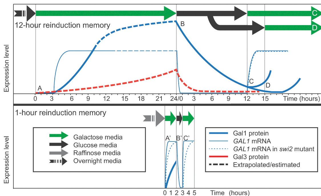
Fig. 2 Timecourses of reinduction memory experiments. Top: 12-hour reinduction memory. 4,32 Bottom: 1-hour reinduction memory. 20 Timecourse curves are approximate. GAL1 and GAL3 mRNA and proteins are not on the same vertical scale. (A) Primary induction after overnight glucose. (A') Primary induction after overnight raffinose. (B, B') Glucose repression. (C) Secondary induction after 12 hours is faster than primary induction. (C') Secondary induction after 1 hour is faster than primary induction for wild-type. Secondary induction is the same as primary induction (A') for swi2Δ , indicating loss of the memory phenotype in the mutant. (D) Secondary induction after 15 hours is as slow as primary induction. Data sources ("WT" = wild-type): (A) Gal1p: 4 Fig. 1c, 14 Fig. 6. GAL1 WT: 32 Fig. 1a. (A') Gal1p: 58 Fig. 4, in a neutral medium similar to raffinose. GAL1 WT: 20 Fig. 6 ( GAL1 ) and Fig. 2 ( GAL10 , similar). GAL1 swi2Δ : 20 Fig. 6. (B, B') Gal1p: 4 Fig. S3A. GAL1 : 33 Fig. 2c. (C) Gal1p: 4 Fig. 1c. GAL1 WT: 32 Fig. 1c, 20 Fig. 1a. GAL1 swi2Δ : 20 Fig. 1b. (C') GAL1 WT: 20 Fig. 6 ( GAL1 ), Fig. 2 ( GAL10 , similar). GAL1 swi2Δ : 20 Fig. 6c. (D) Gal1p: 4 Fig. S3B.
